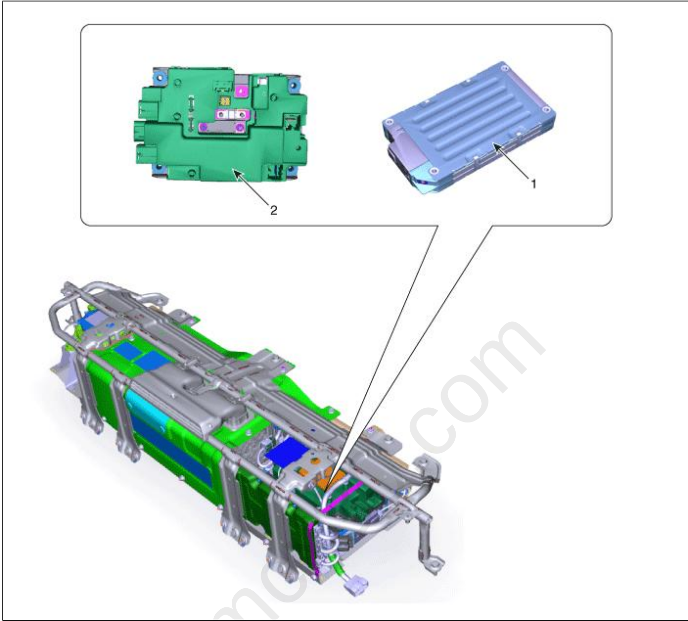
1. Auxiliary 12V battery
